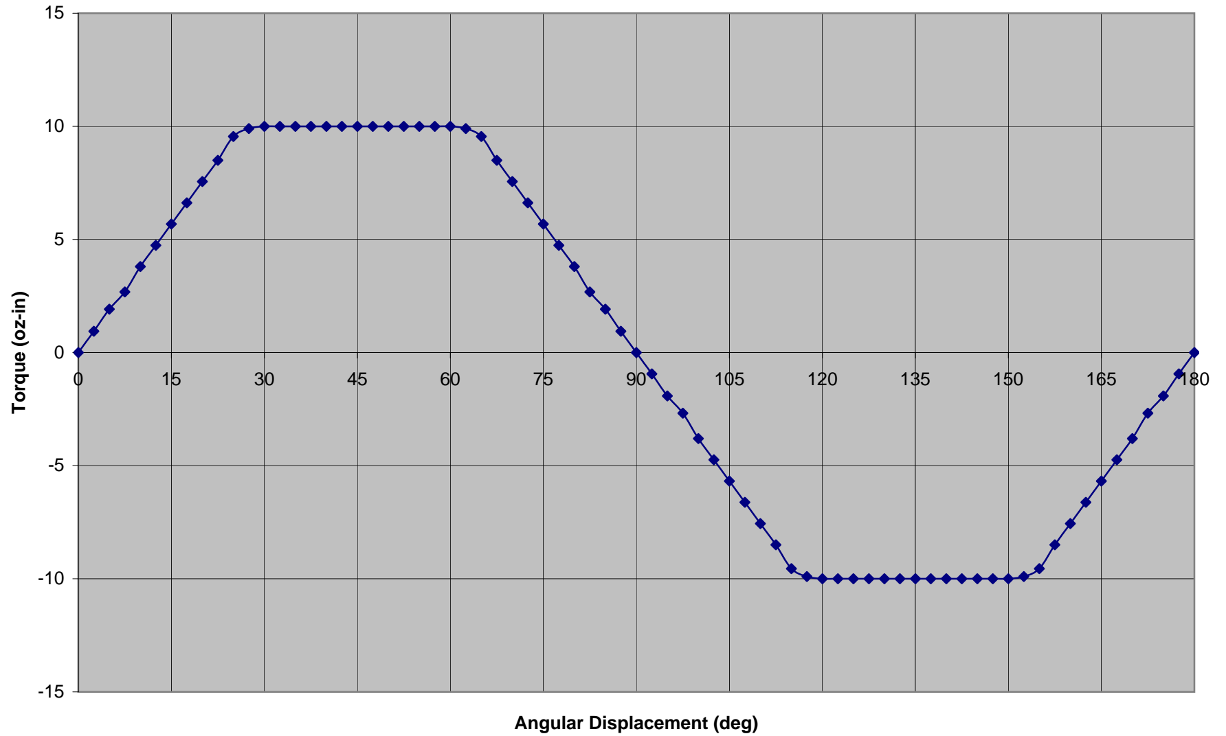
Torque vs. Displacement (TMR-020-010-4)
