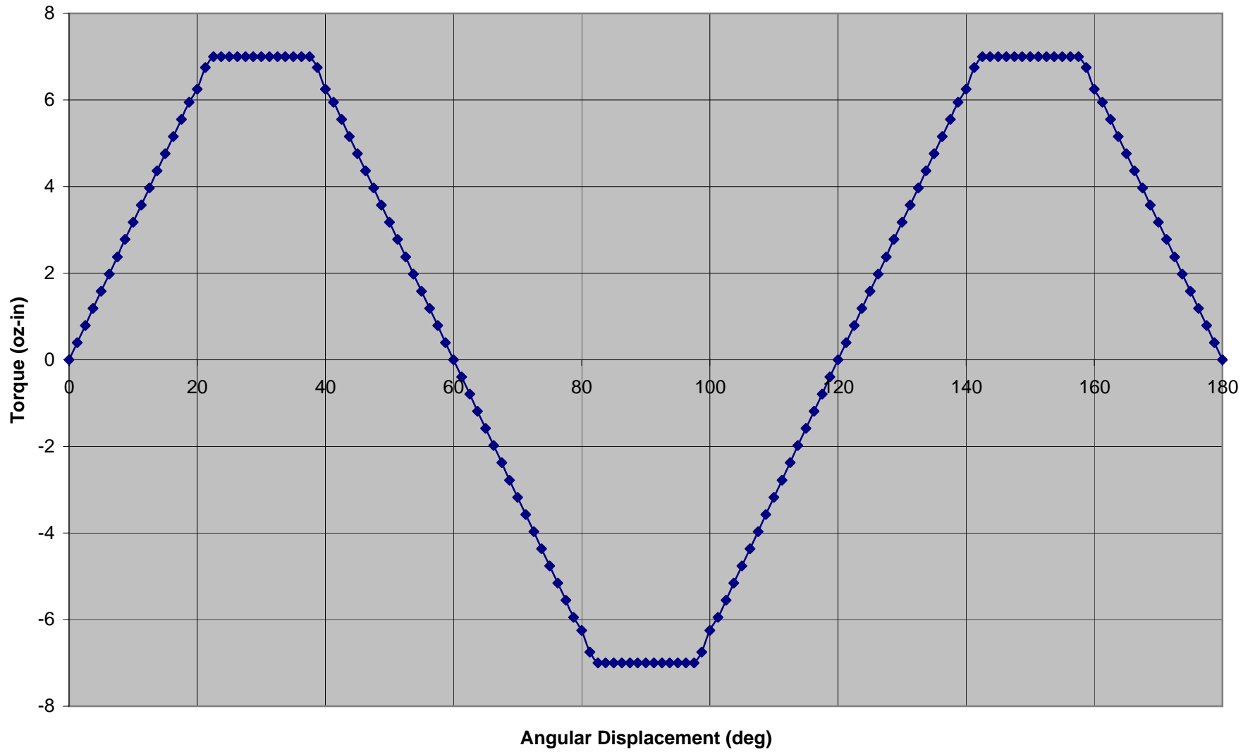
Torque vs. Displacement (TMR-016-007-6)
